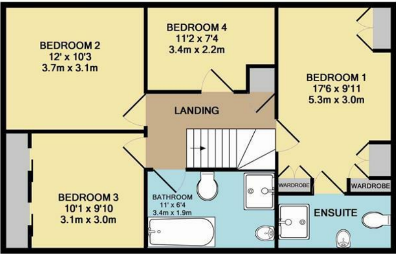
1ST FLOOR
